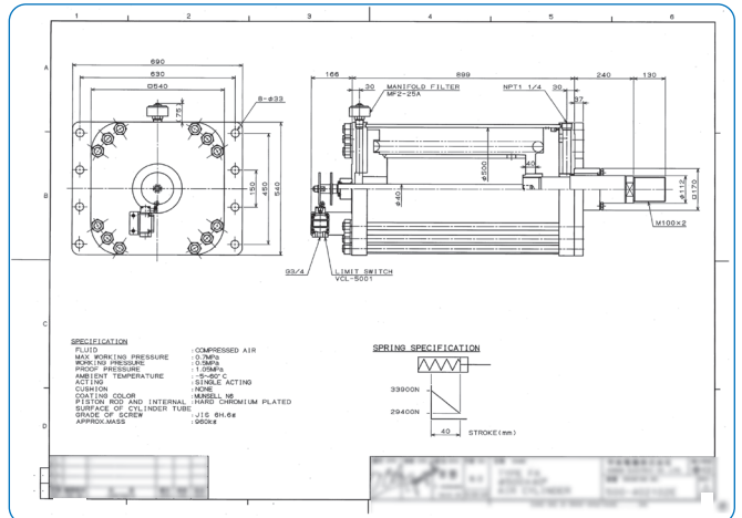
[φ500×40 S 単動引込形]
