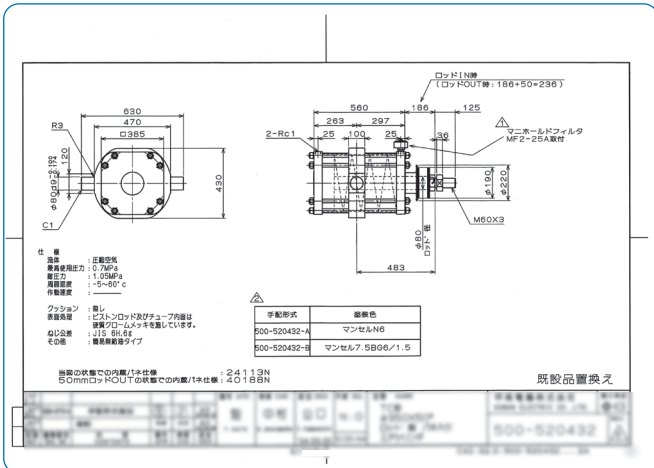
[φ350×50 S 単動押出形]
