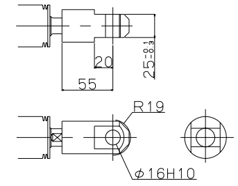
Y-Type Rod Joint
