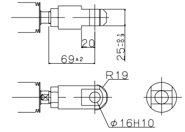
Y-Type Rod Joint
