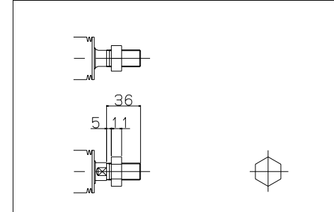
Lock Nut
